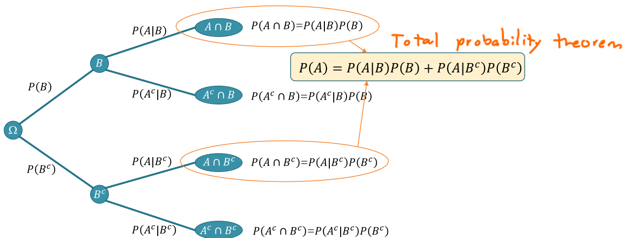
Figure 6: Tree Diagram and Conditional Probabilities
